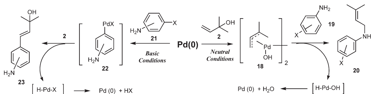
Scheme 3. Pathway of the palladium-catalyzed reaction of haloaniline 21 .
