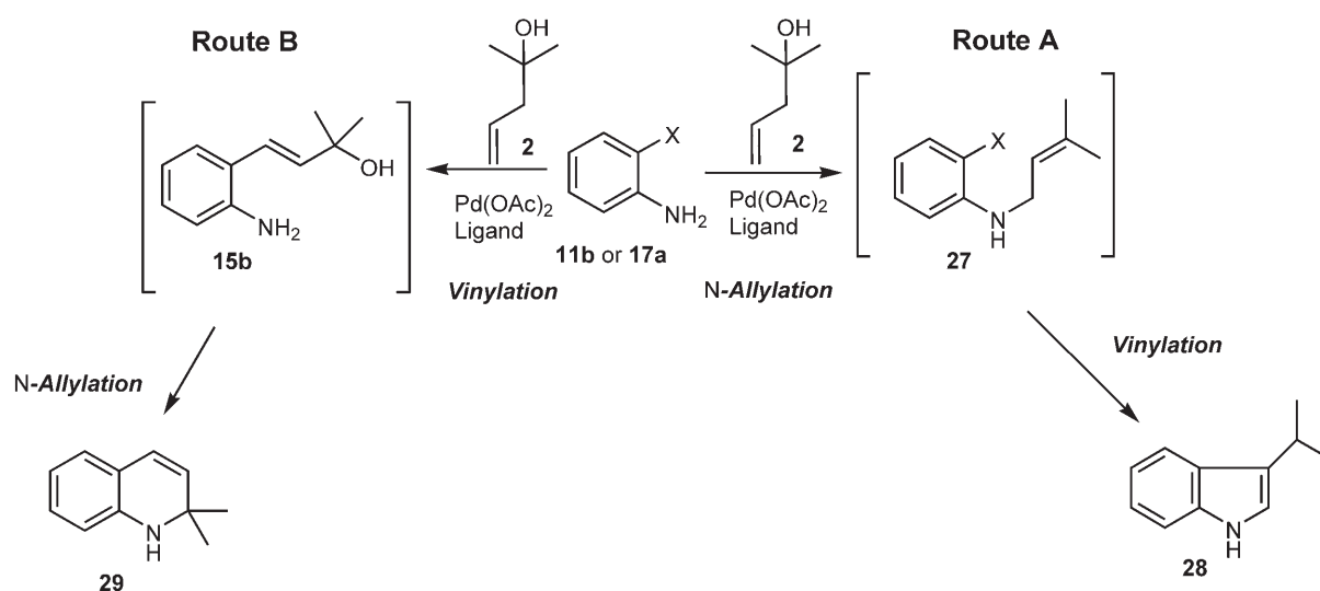
Scheme 4. Synthetic plan for heterocycles.
