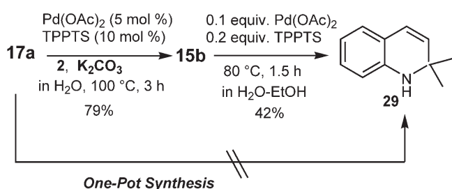
Scheme 6. One-pot synthesis of 2,2-dimethylquinoline 29 .
