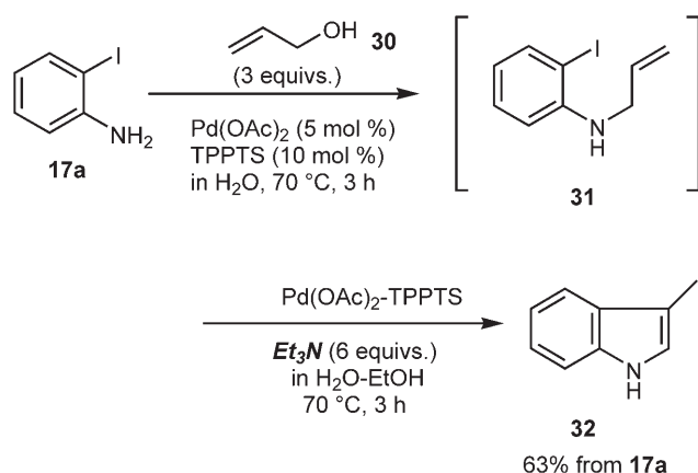
Scheme 5. One-pot synthesis of 3-methylindole 32 .
