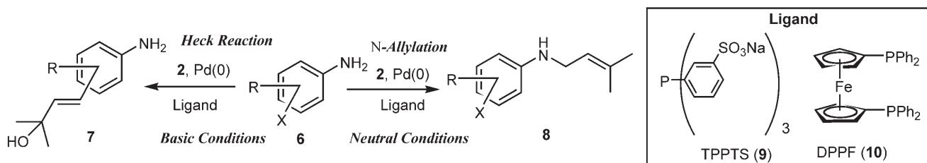
Scheme 2. Palladium-catalyzed chemoselective reaction of haloanilines 6 .
